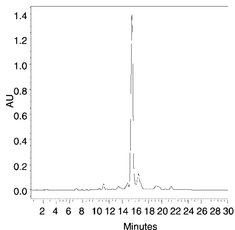
Figure 5. HPLC profile of trimer Dmtr-C Bz pScneA Bz pScneG iBu -3'-OH.
