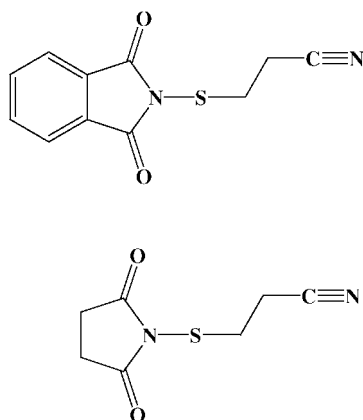
Figure 3. Reagents used for the oxidation of the H -phosphonate diester linkage.
