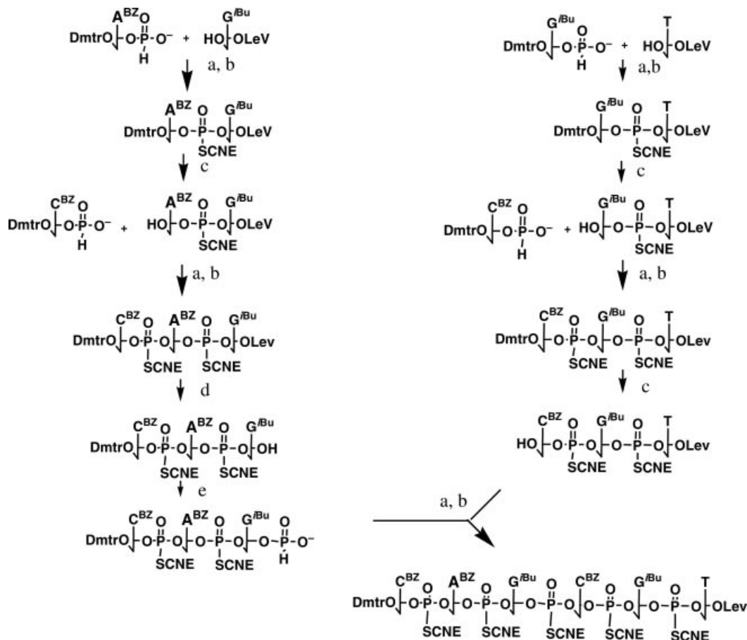
Scheme 5. Convergent synthesis of fully protected hexamer CAGCGT. Reagents and conditions: a. acyl chloride resin, CH_2Cl_2 , pyridine; b. succ- S -CNE; c. 2% BSA, CH_2Cl_2/MeOH ; d. hydrazine resin; e. salicylchlorophosphite, CH_2Cl_2 , pyridine.
