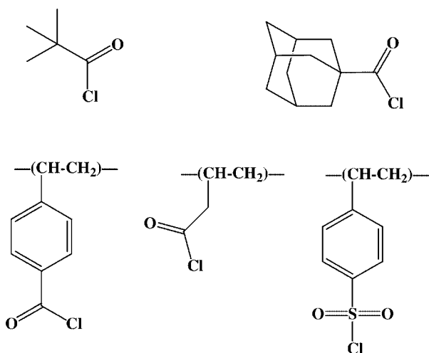
Figure 1. Soluble and solid-supported acyl and sulfonyl chlorides.
