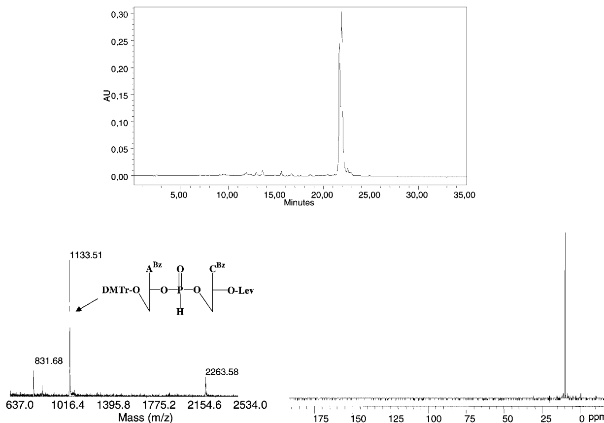
Figure 2. HPLC profile, MALDI-TOF MS and 31 P NMR spectra of dimer Dmtr-dA Bz -HP-dC Bz -3'-Lev after precipitation.
