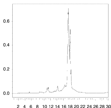
Figure 6. HPLC profile of trimer DmtrC Bz pScneA Bz pScneG iBu -3'-HP.
