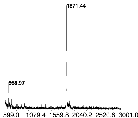
Figure 7. HPLC profiles of fully protected (left) and deprotected (right) hexamer CAGCGT and MALDI-TOF MS of deprotected hexamer.
