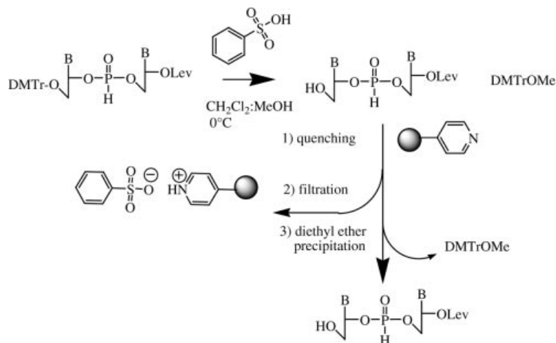
Scheme 4. Schematic protocol for detritylation with benzenesulfonic acid and quenching with PVP resin.
