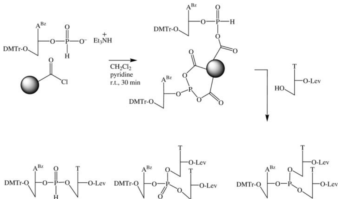
Scheme 3. Overactivation of H -phosphonate monoester by acyl chloride resin.
