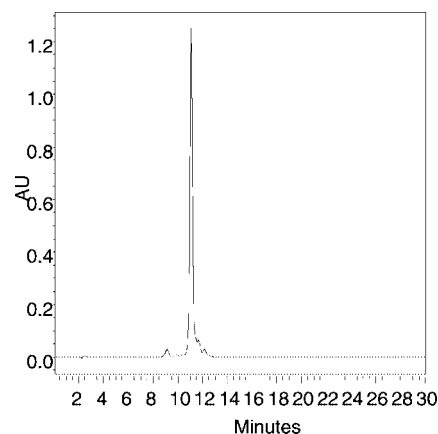
Figure 4. HPLC profile of 5'-OH- C^{Bz}pS_{CNE}G^{iBu}pS_{CNE}T-Lev after precipitation.
