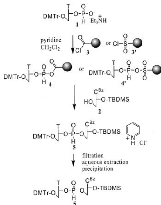
Scheme 2. Synthesis of the dimer H -phosphonate diester through the H -phosphonate SOLIGO process.
